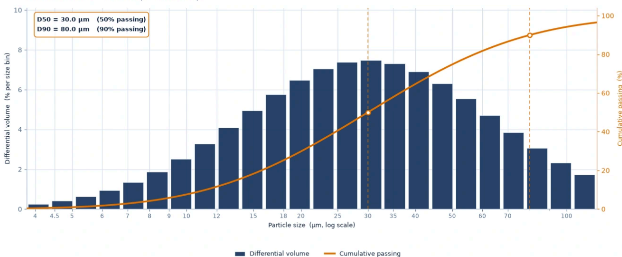
Particle Size Distribution — KAO-KTB
